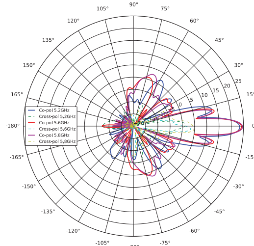
V-POL Azimuth Gain (dBi) or Zero Elevation
