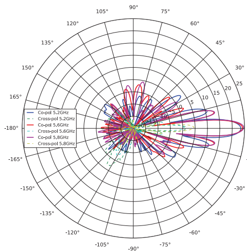
V -POL Elevation Gain (dBi) for Zero Azimuth
